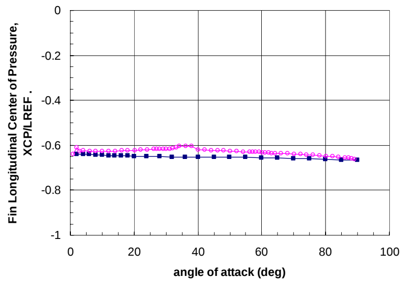
Figure 16. Fin Longitudinal Center of Pressure for T2.
