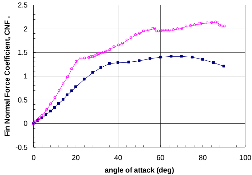
Figure 12. Normal Force Coefficient for T1.
