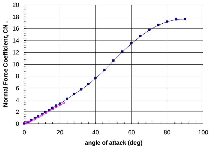
Figure 22. Normal Force Coefficient for B7T5.
