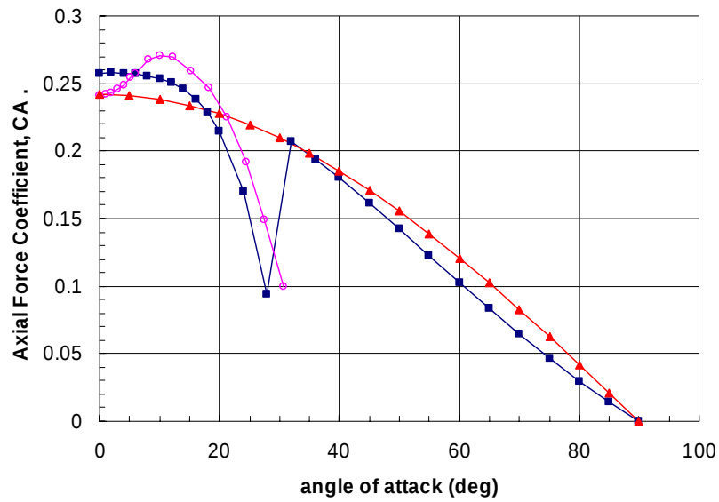
Figure 10. Axial Force Coefficient for B5.
