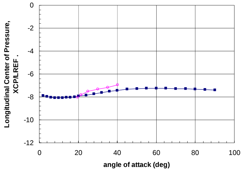
Figure 25. Longitudinal Center of Pressure for B8T6.
