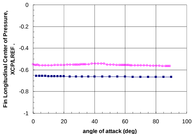
Figure 17. Fin Longitudinal Center of Pressure for T4.
