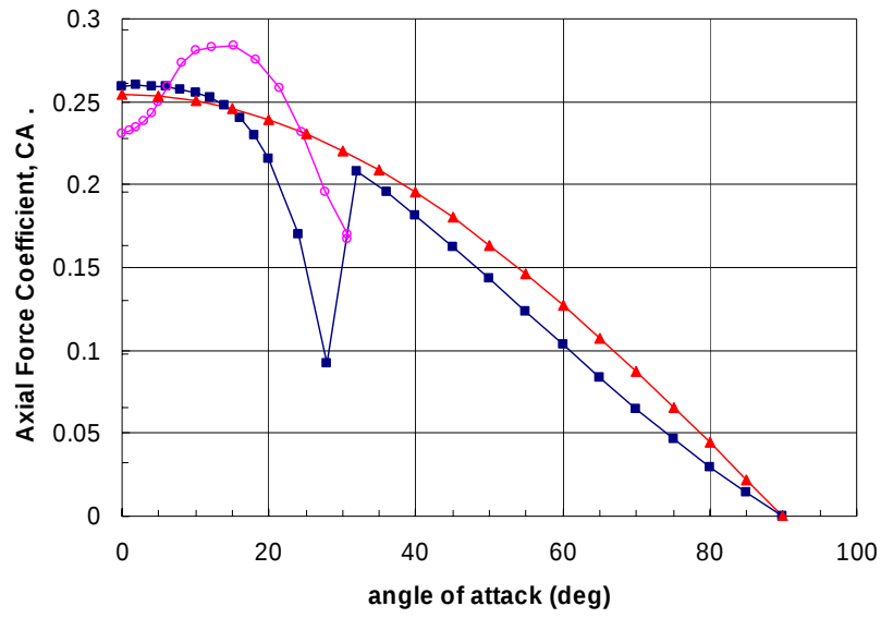
Figure 9. Axial Force Coefficient for B1.
